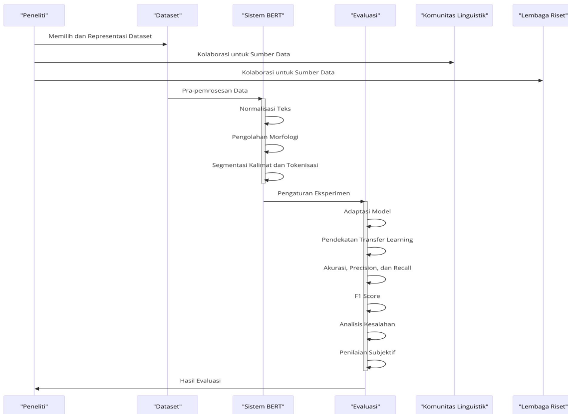
Gambar 1. Diagram alur metodologi penelitian
