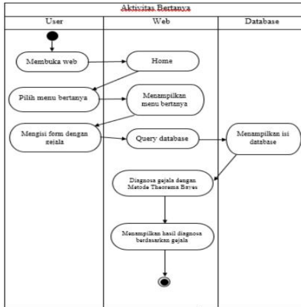
Gambar 3. Activity Diagram
