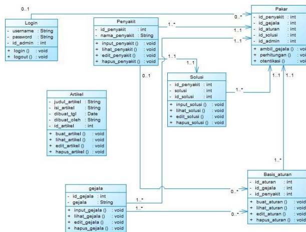
Gambar 4. Class Diagram
